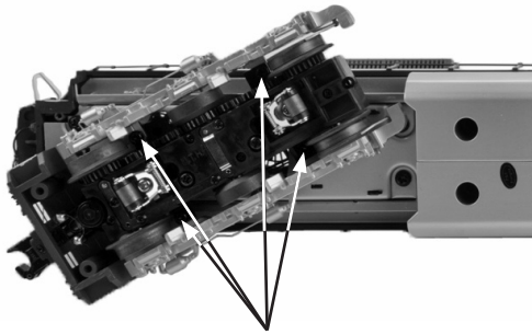
Truckside Screws
