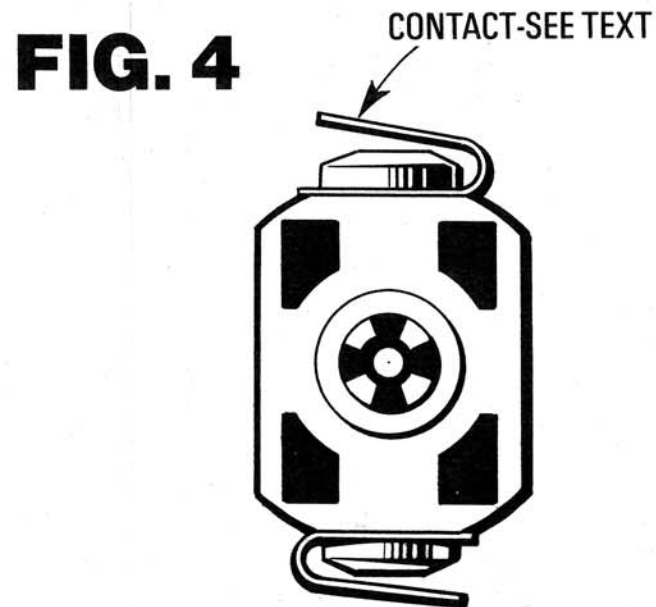
Brush Contact Arrangement
